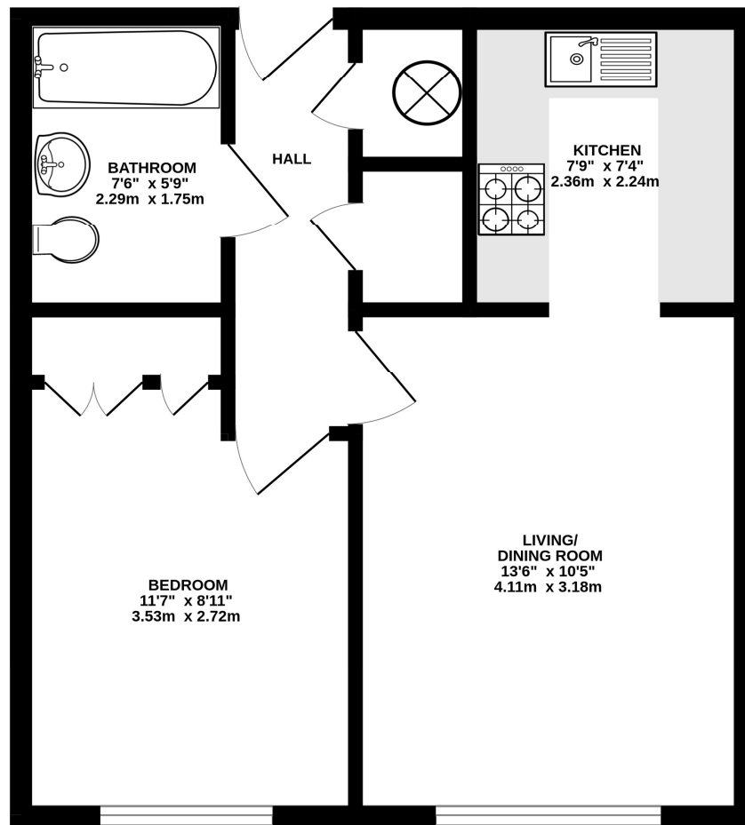
SECOND FLOOR FLAT
