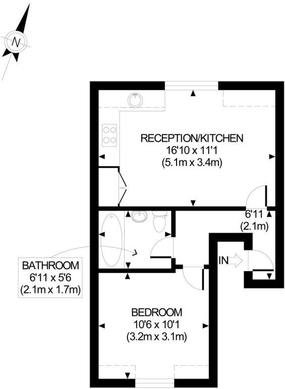
SECOND FLOOR GROSS INTERNAL FLOOR AREA 385 SQ FT
