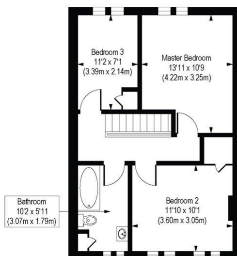
First Floor Gross Internal Floor Area 504 sq ft
