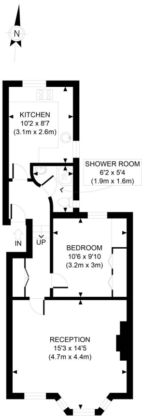
FIRST FLOOR GROSS INTERNAL FLOOR AREA 504 SQ FT
