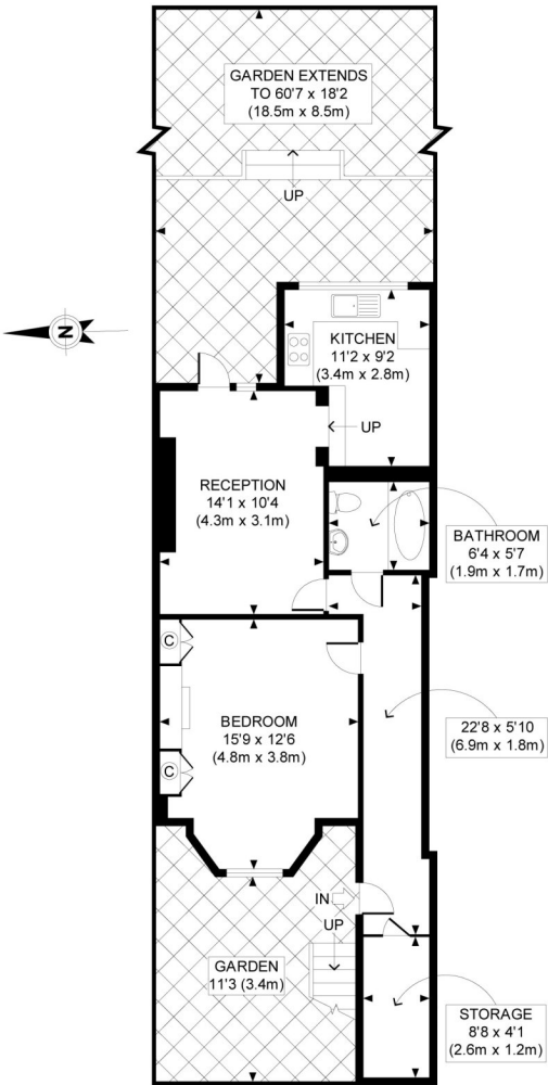
GROUND FLOOR GROSS INTERNAL FLOOR AREA 603 SQ FT APPROX. GROSS INTERNAL FLOOR AREA 603 SQ FT / 56 SQ M Ref: WWSBL - 050312 Copyright photoplan.co.uk Floorplans are for identification and guideline purposes only, not to scale. Compliant with RICS code of measuring practice.
