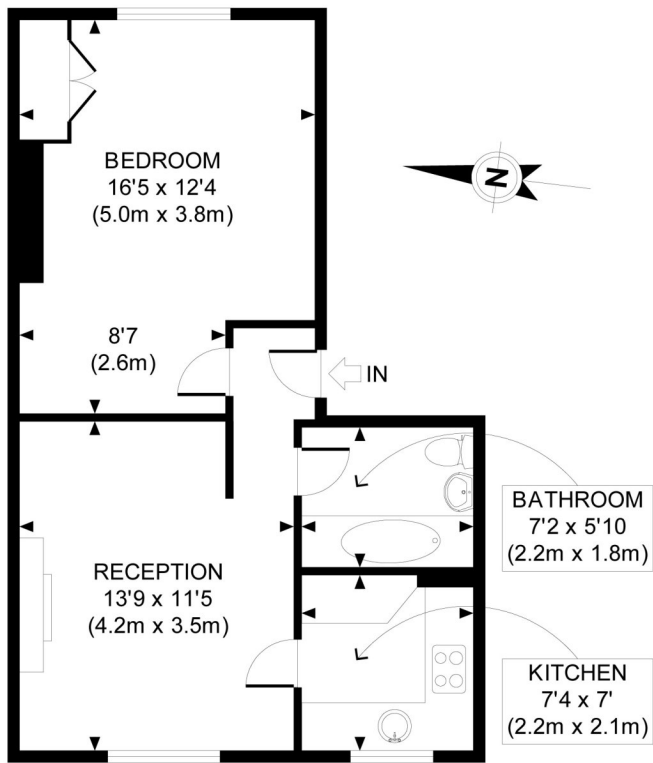
FIRST FLOOR GROSS INTERNAL FLOOR AREA 463 SQ FT
