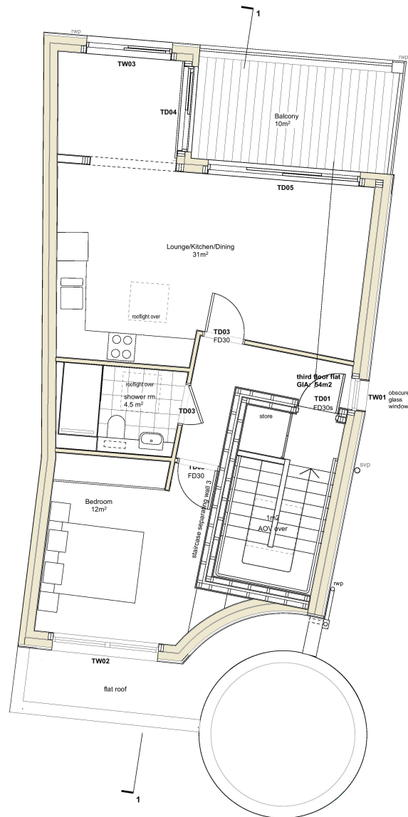
6 THIRD FLOOR PLAN (NEW FLAT) Scale: 1:50
