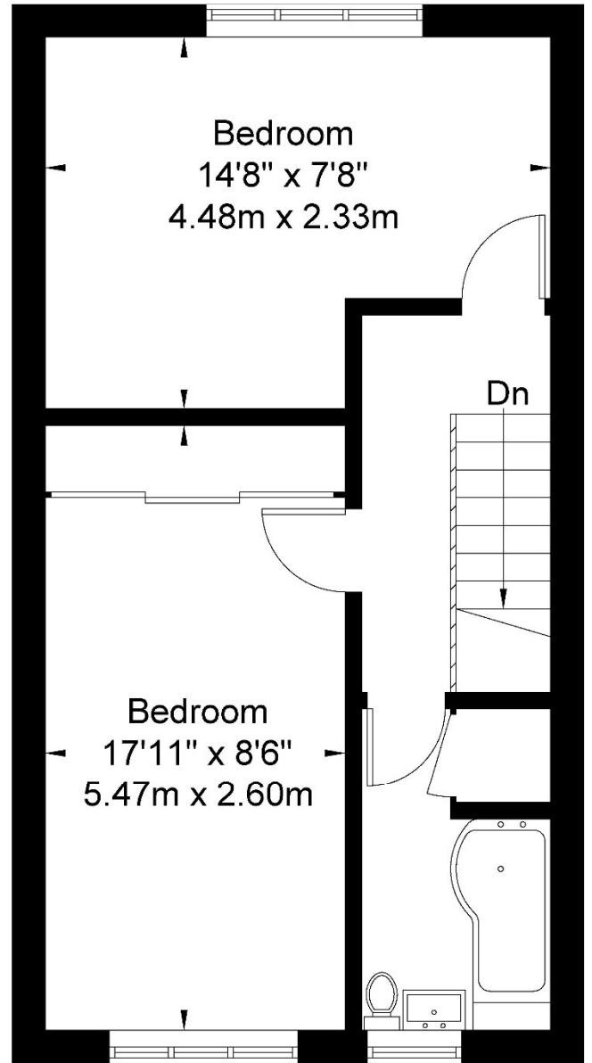
Second Floor
