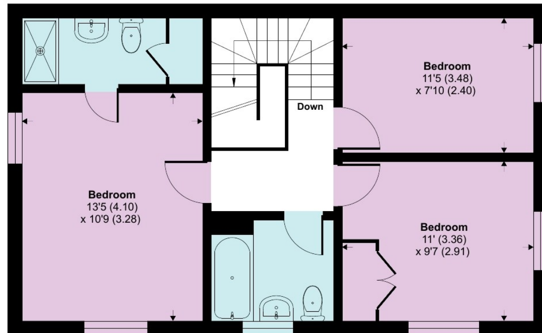
FIRST FLOOR
