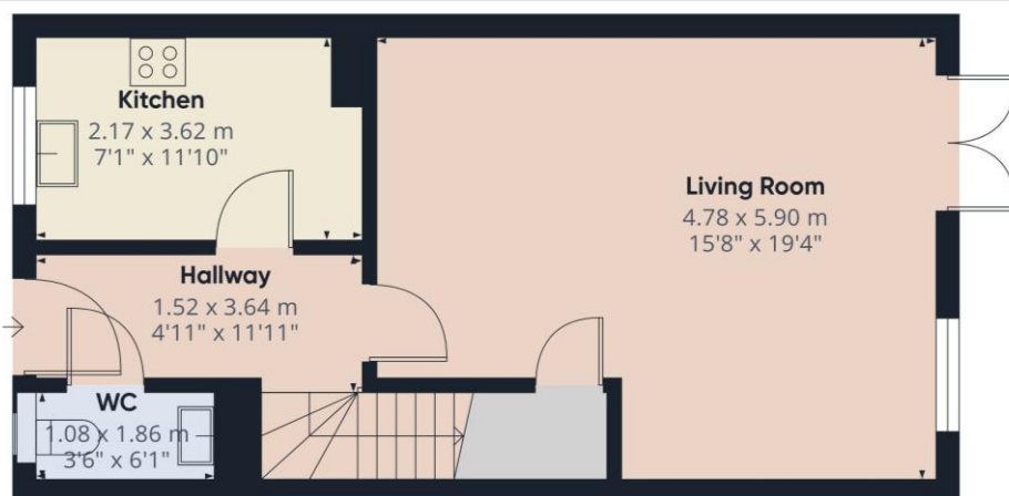
Ground Floor
