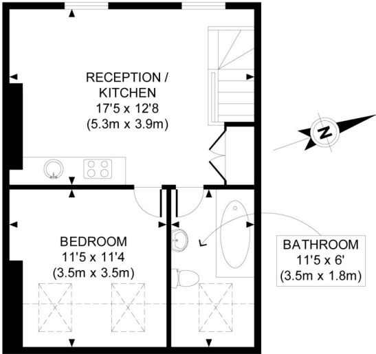
THIRD FLOOR GROSS INTERNAL FLOOR AREA 431 SQ FT
