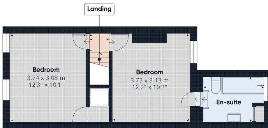
Floor 1
