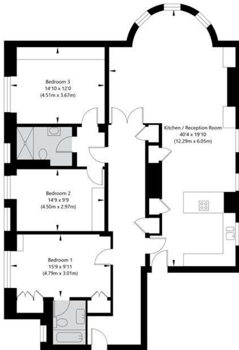
Raised Ground Floor GROSS INTERNAL FLOOR AREA APPROX. 139.02 SQ M / 1496 SQ FT
