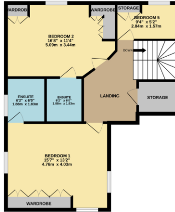
1ST FLOOR 670 sq.ft. (62.2 sq.m.) approx.
