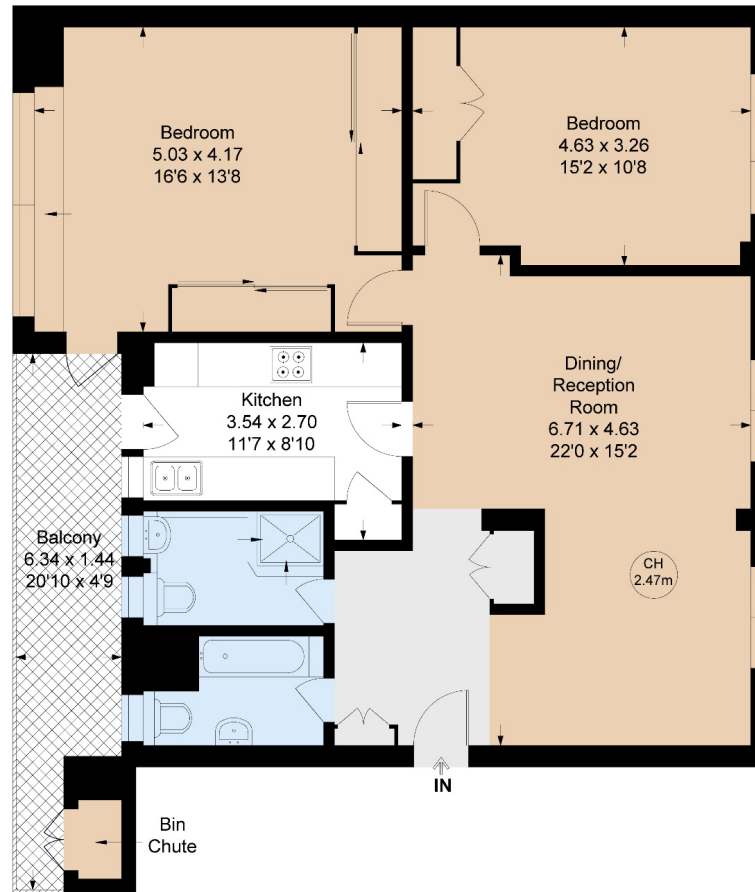
Fifth Floor
