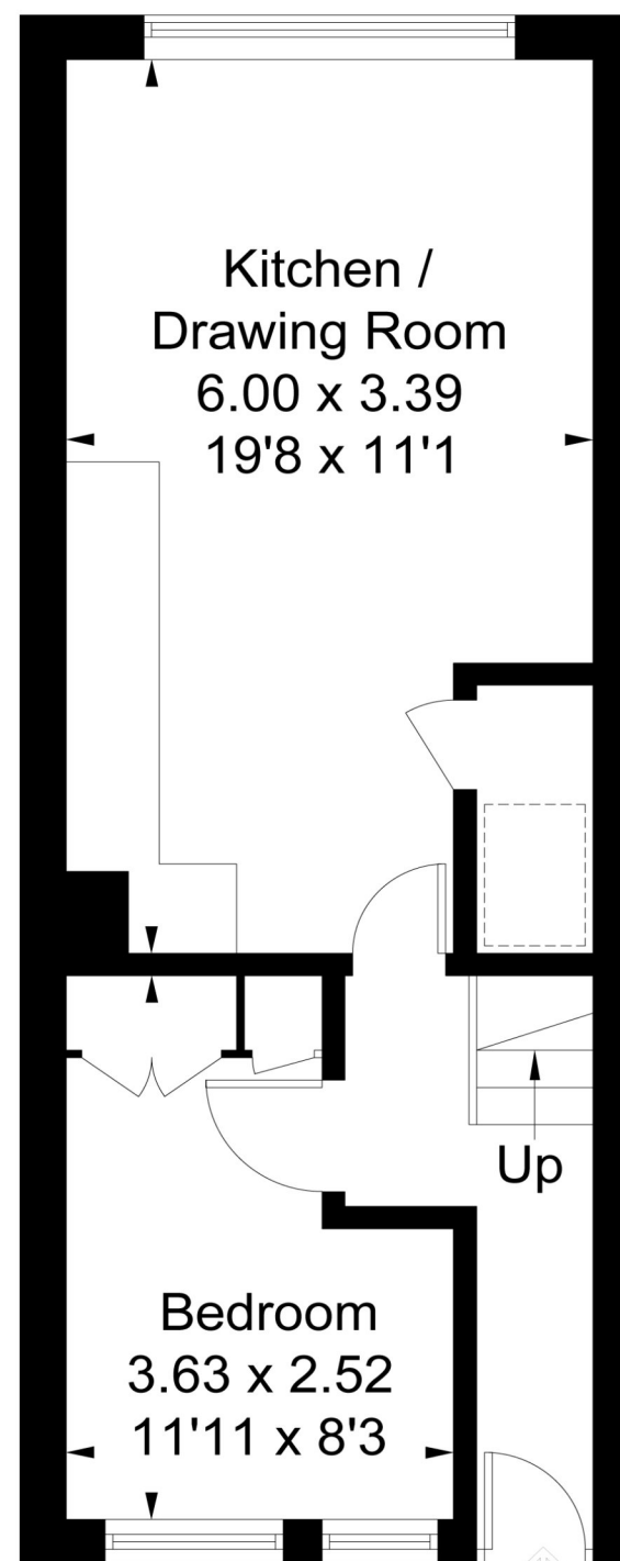
Ground Floor
