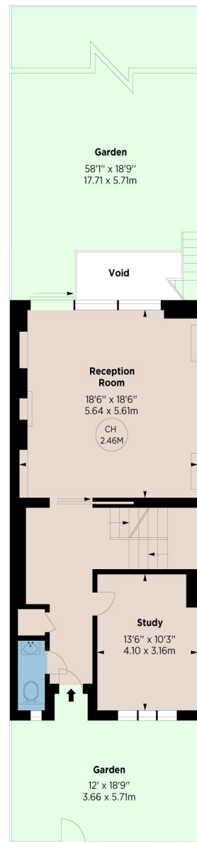
GROUND FLOOR
