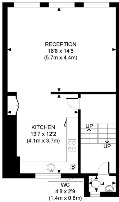
SECOND FLOOR GROSS INTERNAL FLOOR AREA 547 SQ FT
