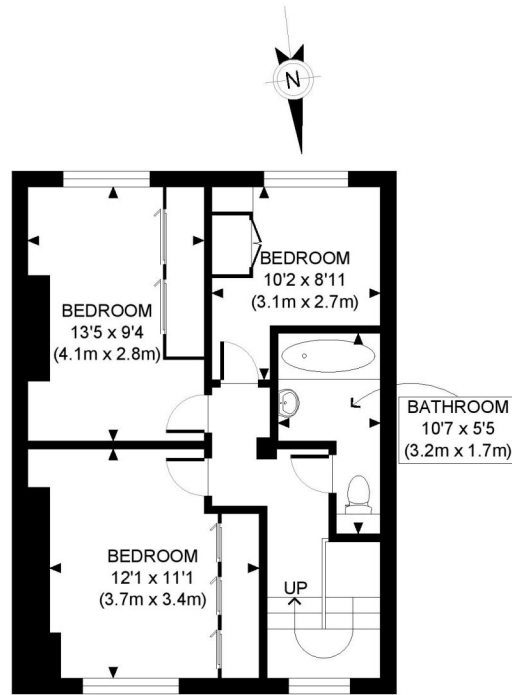
THIRD FLOOR GROSS INTERNAL FLOOR AREA 484 SQ FT
