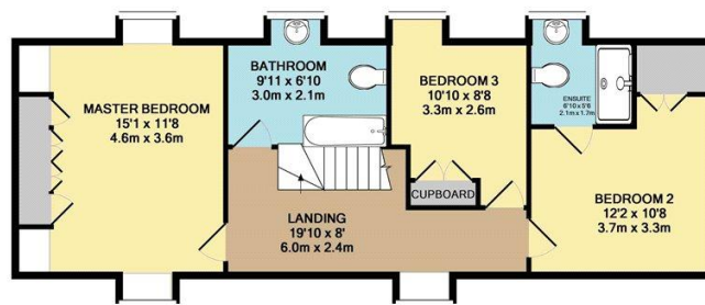
1ST FLOOR
