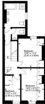
Second Floor
