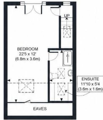
SECOND FLOOR GROSS INTERNAL FLOOR AREA WITH EAVES 388 SQ FT FLOOR AREA WITHOUT EAVES 339 SQ FT
