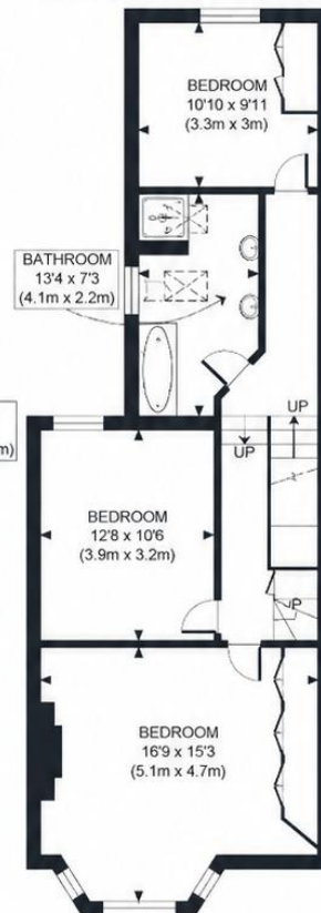
SECOND FLOOR GROSS INTERNAL FLOOR AREA WITH EAVES 388 SQ FT FLOOR AREA WITHOUT EAVES 339 SQ FT
