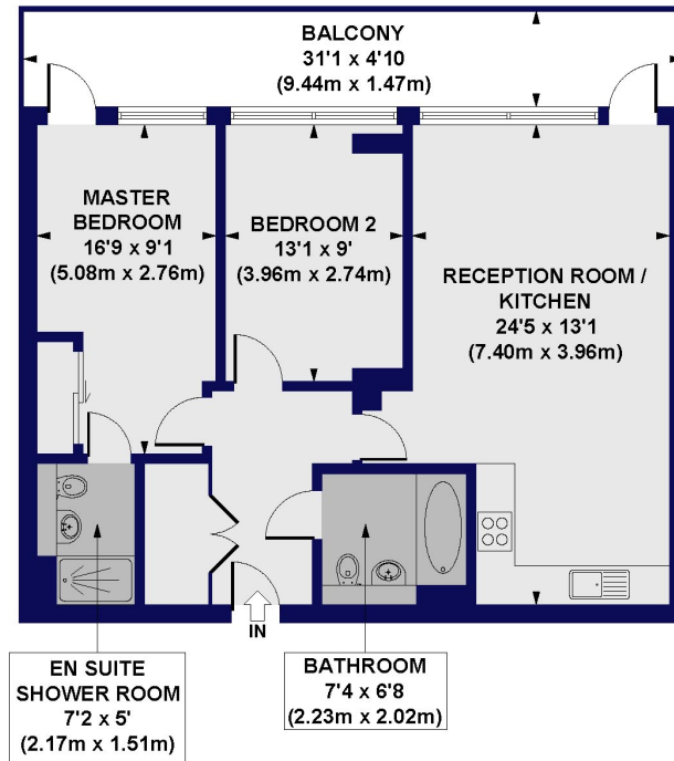
THIRD FLOOR
