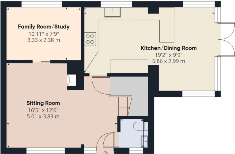
Ground Building 1
