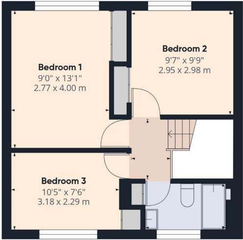
Floor 1 Building 1
