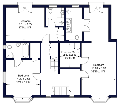
First Floor Sq m 106.4 / Sq ft 1145
